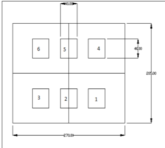
Fig. 2 Selected Location of Modules on a Aluminium plate
