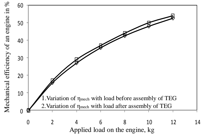
Fig. 4 Variation of mechanical efficiency with applied load
