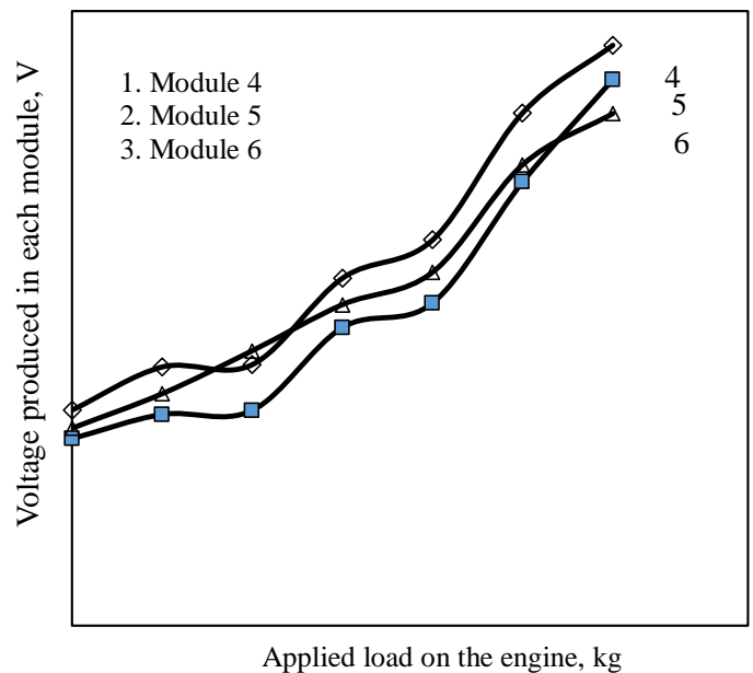
Fig. 6 Variation of voltage with applied load for modules 4, 5, 6
