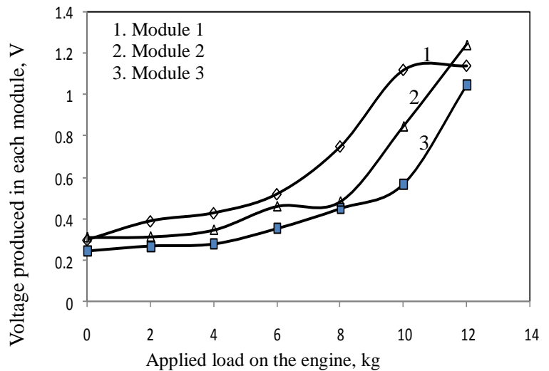
Fig. 5 Variation of voltage with applied load for modules 1, 2, 3
